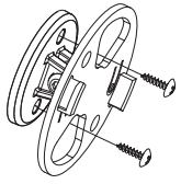
STEP 1: Fix the body to the wall with the 2 provided screws
