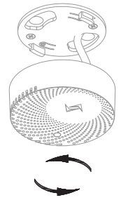
STEP 2: Clip the body onto the main base plate.
